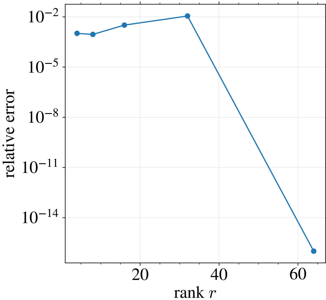
Haar covariance relative error
