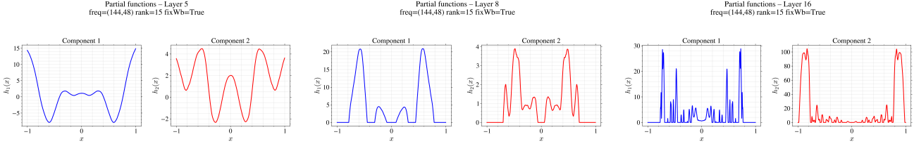
Figure 9. (symmetric) with bigger spikes. (a) f_1^{(5)} . (b) LeakyReLU( H_8 ) (c) LeakyReLU( H_{16} ).
