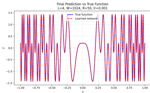
Figure 7. Final prediction vs. target f(x) = \cos(36\pi x^2) - 0.8 \cos(12\pi x^2) . 4-layer, n=1024 , r=50 , N=1000 , RF-LR MSEs are within 10^{-8} to \sim 10^{-4}
