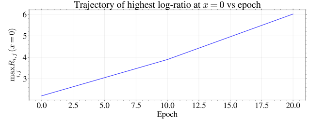
Figure 5. Trajectory of \max_{i,j} R_{i,j}(x=0) vs. epoch (layer-3 channels). Channel specialization at x=0 as in Theorem 4.1. Setup: n = 1024 , r = 15 , \cos(8\pi x) , 20 epochs.
