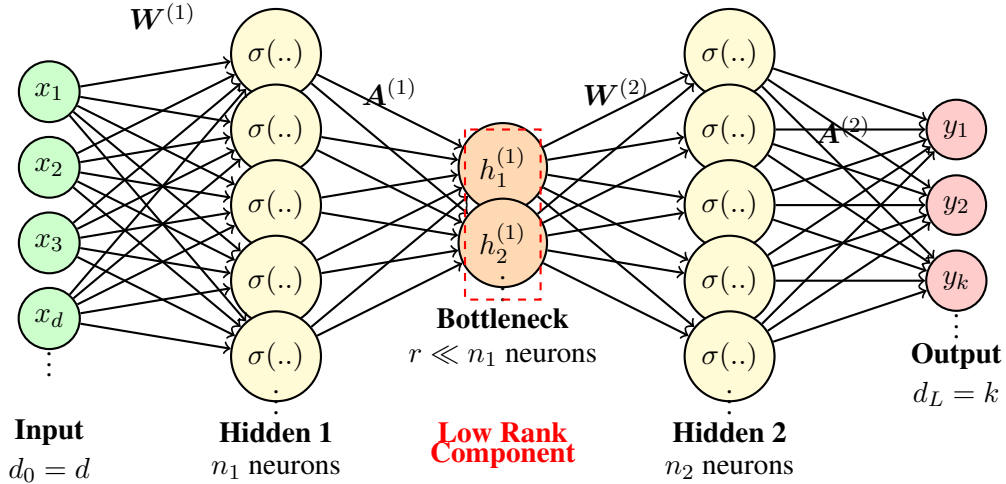
Figure 1: Architecture of a Multi-component Multi-layer Neural Network (RF-LR). The red dashed connections indicate the low-rank component that reduces dimensionality from n_1 to r \ll n_1 neurons. We only train the output weights A^{(1)} and A^{(2)} .
