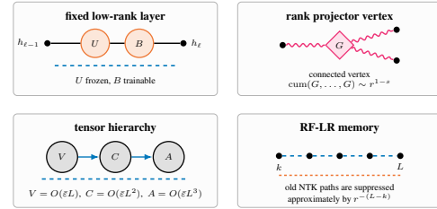
Figure 2. Main diagrammatic objects. Solid black lines denote NNGP/preactivation transport, dashed blue lines denote NTK legs, orange vertices denote low-rank factors, pink diamonds denote Stiefel-projector cumulants, and gray blobs denote transported tensor cumulants.
