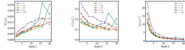
Figure 5. True finite-network cumulants from autodiff NTKs. These scalar-output cumulants are not isolated Feynman coefficients; they test the predicted polynomial control and rank-width scaling on actual finite networks.
