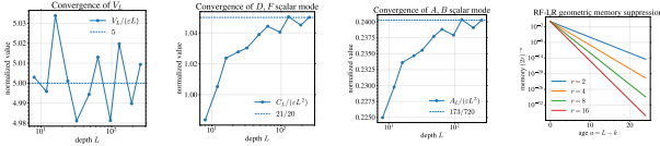
Figure 6. Tensor constants and RF-LR memory. The first three panels show convergence to the isolated constants 5, 21/20, and 173/720. The last panel shows geometric suppression of old NTK memory in the RF-LR bottleneck.
