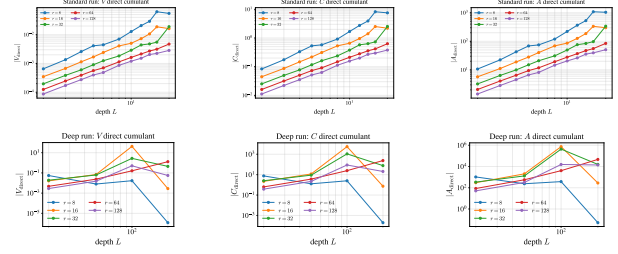
Figure 8. Log-log finite-network cumulant magnitudes. Top: the standard long run. Bottom: the L \in \{20, 50, 100, 200\} deep stress test. These plots show effective depth slopes directly, before normalizing by the proposed L , L^2 , and L^3 scales.
