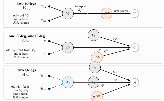
Figure 3. Diagrammatic reduction of the tensor hierarchy. External K - and \Theta -legs choose the block being computed. Connected terms either transport an older tensor, feed a lower block into a higher one, or create a fresh low-rank source \Xi .
