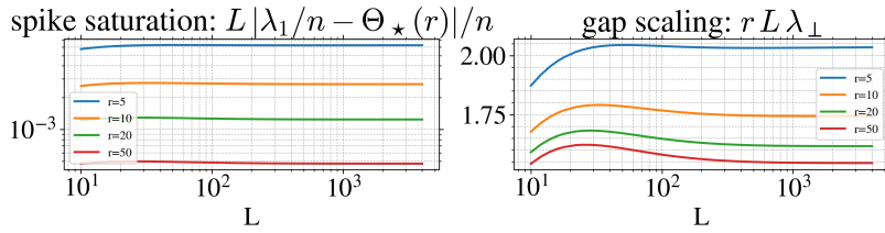
Figure 6: Equicorrelated spectrum (Corollary 8): (1) spike saturation L|\lambda_1/n - \Theta_*(r)|/n vs L (log-log); (2) gap scaling rL\lambda_\perp vs L (log-log). One curve per r .
