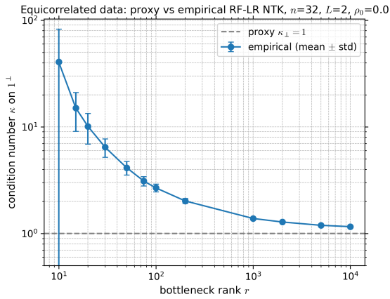
Figure 13: * Equicorrelated: proxy 1; empirical concentrates.
