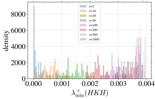
Figure 10: * Histograms of \lambda_{\min}^+(HKH) ; matrix stays PSD.
