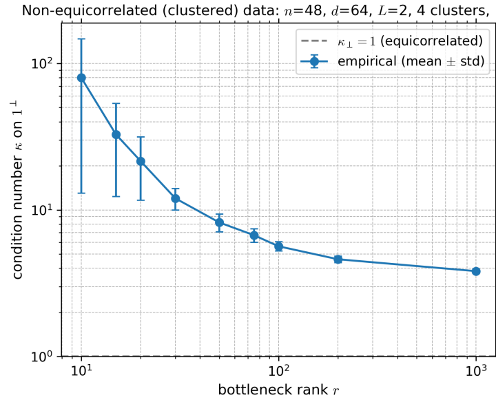
Figure 16: \kappa vs r for clustered (non-equicorrelated) data. \kappa need not approach 1; lower bound \kappa \geq \Omega(r \cdot L) (Proposition 6).
