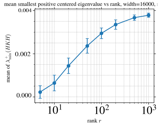
Figure 11: * Mean \lambda_{\min}^+(HKH) vs r ; better conditioning with r .
