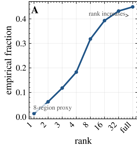
high-codim junctions
