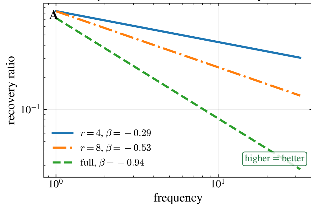
sparse mixture: Fourier recovery
