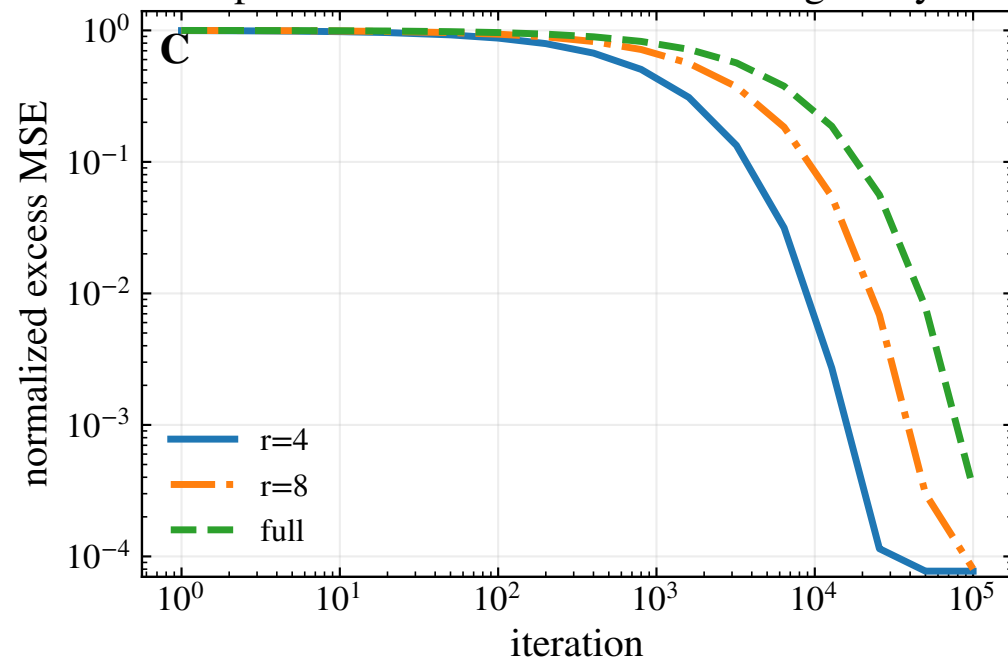
sparse mixture: normalized training decay
