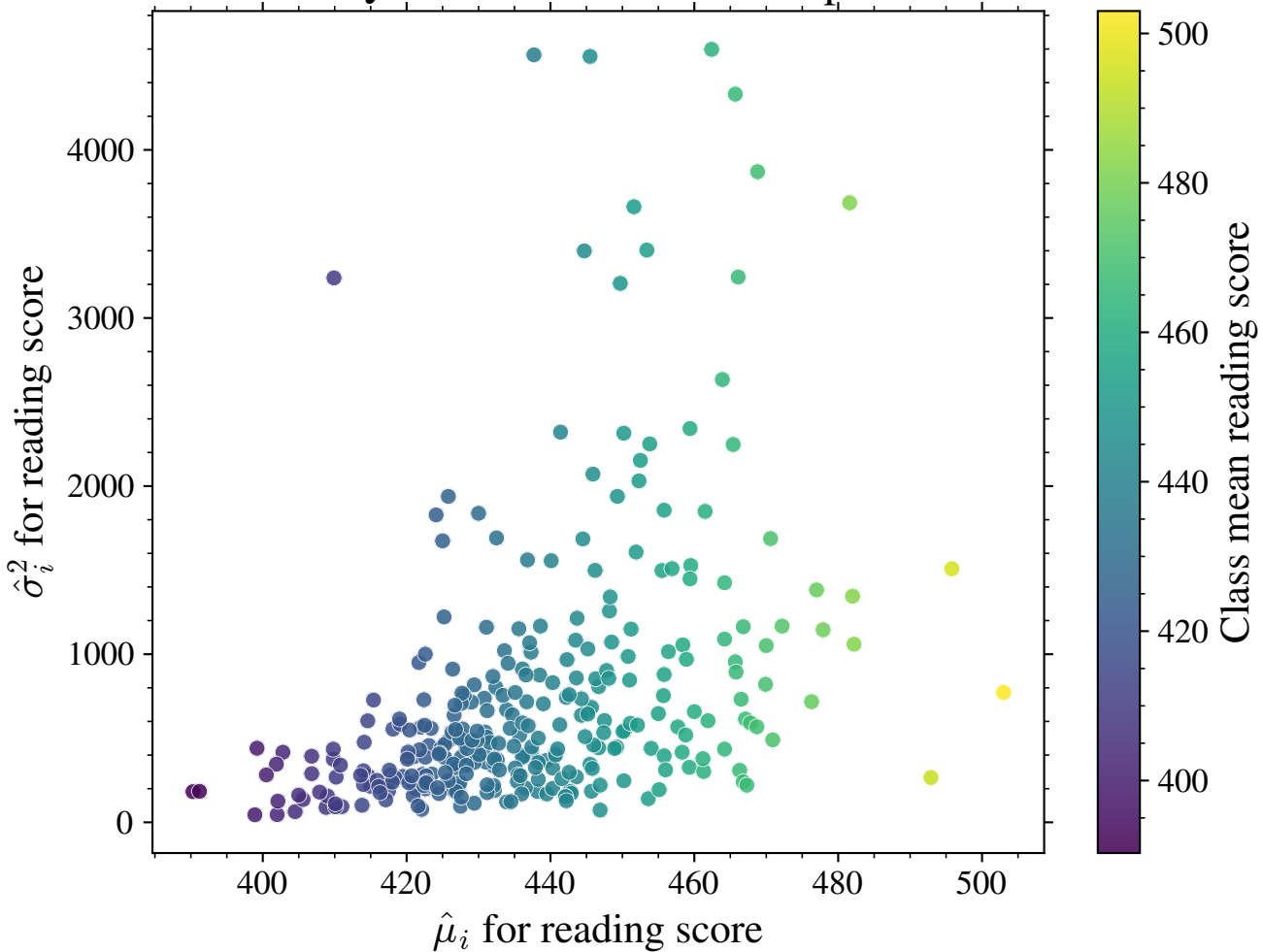
Enriched Q^y : class-level Gaussian parameters
