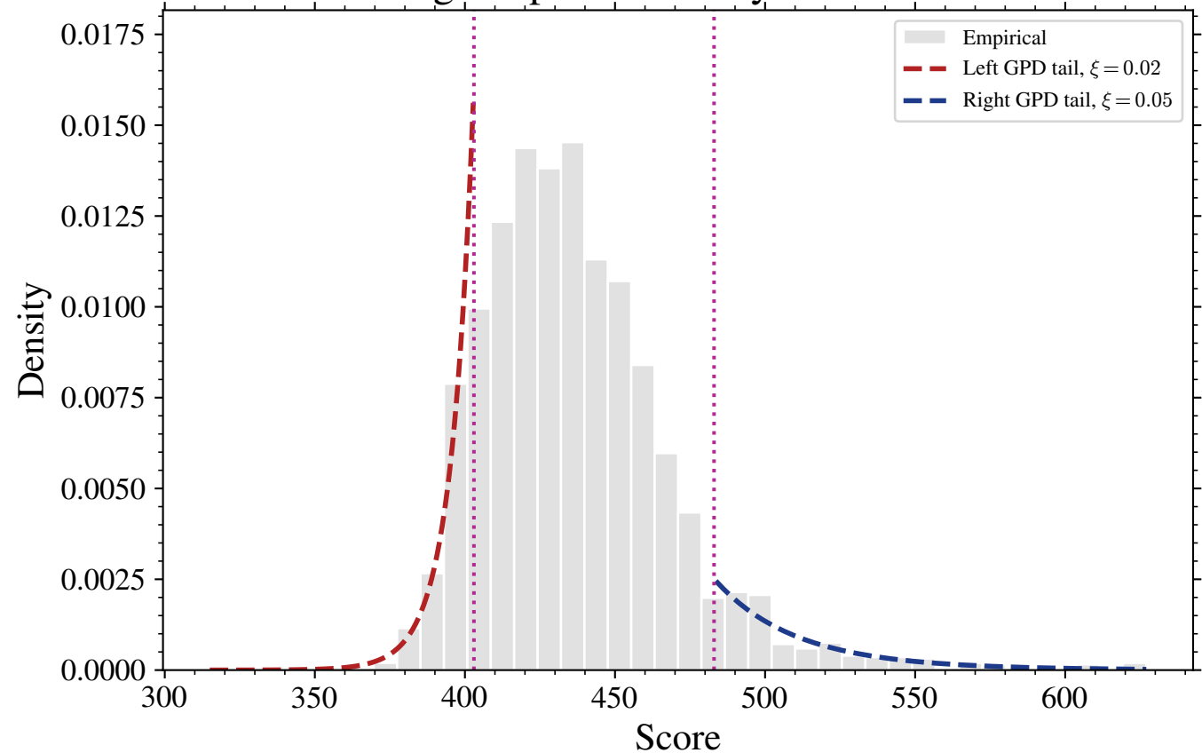
Mathematics: empirical density and left-tail model
