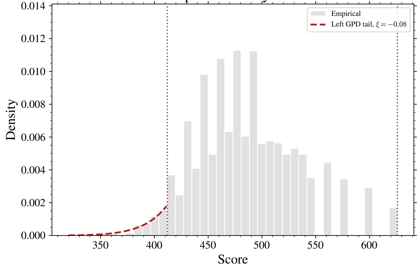
Mathematics: empirical density and left-tail model
