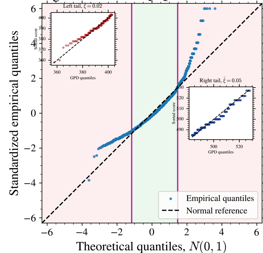
Mathematics: standardized Q-Q with GPD tail zoom
