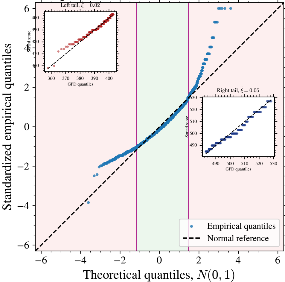
Reading: standardized Q-Q with GPD tail zooms
