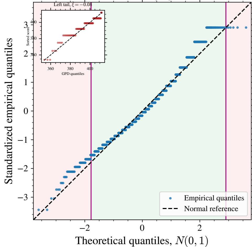
Mathematics: standardized Q-Q with GPD tail zoom
