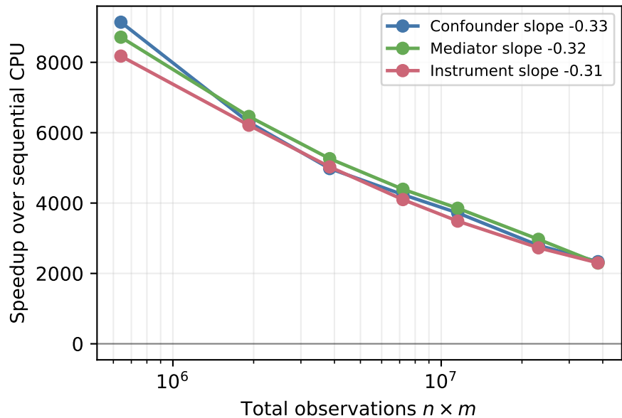
Batched CUDA speedup
