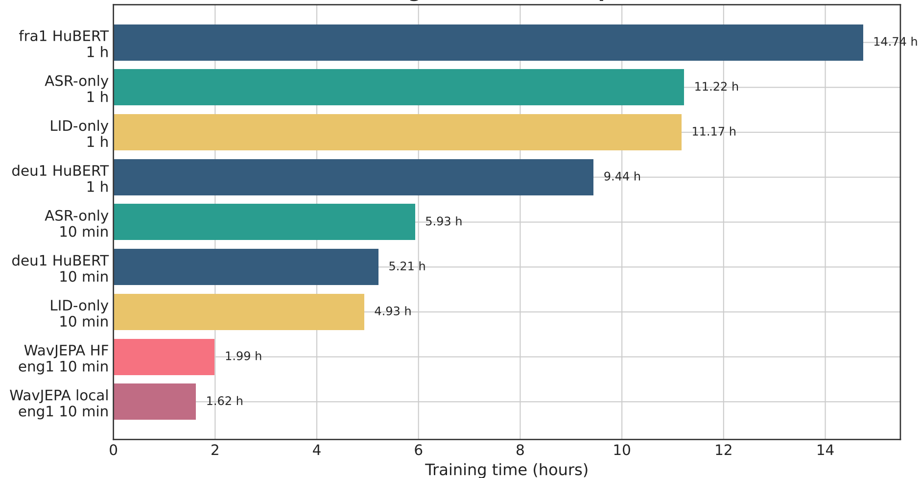
Measured training times across representative runs
