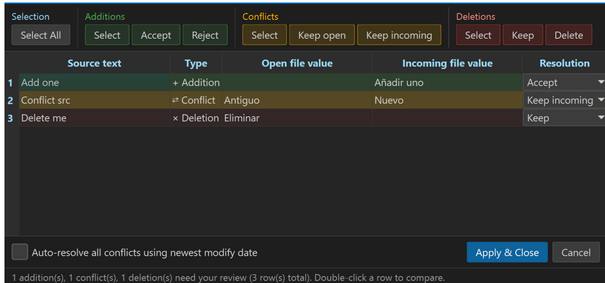
Figure 11 — The Merge dialog, reviewing an addition, a conflict, and a deletion.
