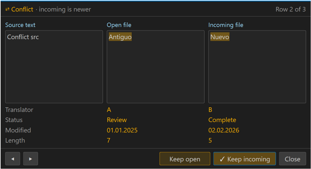
Figure 12 — Comparing one Merge row: the words that differ are highlighted.
