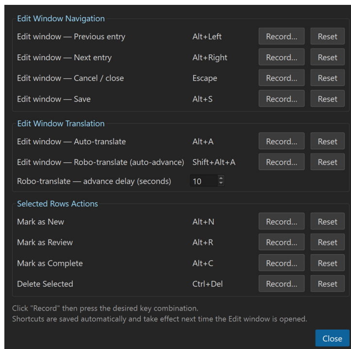
Figure 14 — The Keyboard Shortcuts dialog.
