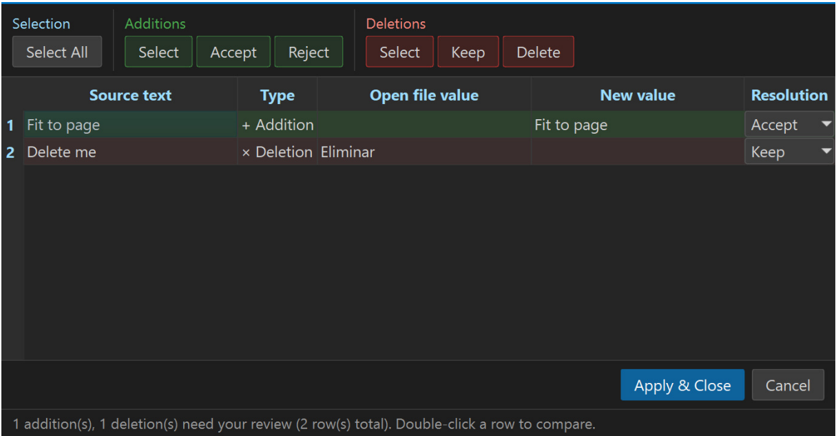
Figure 13 — Sync Keys: additions and deletions only.
