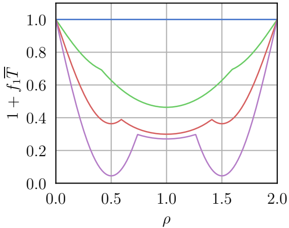
(c) U = W/4
