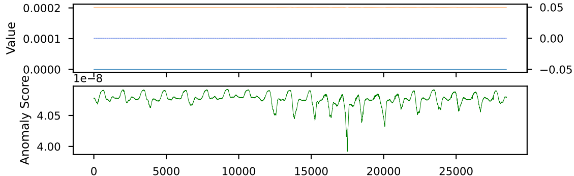
Dimension = 37
