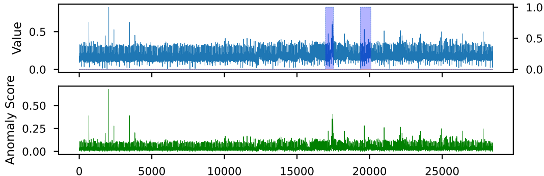
Dimension = 10
