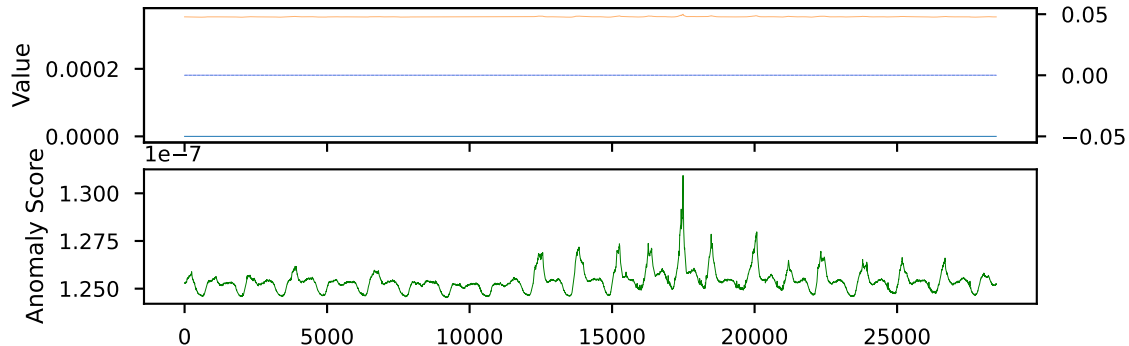
Dimension = 16
