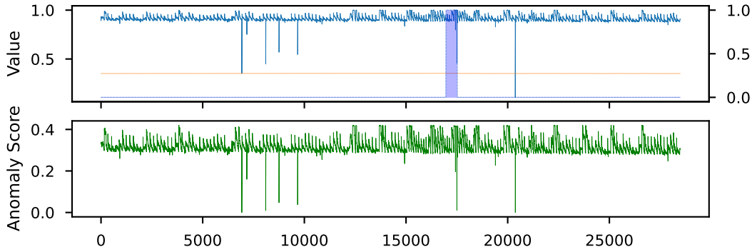
Dimension = 5
