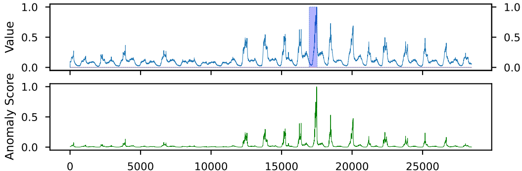
Dimension = 19
