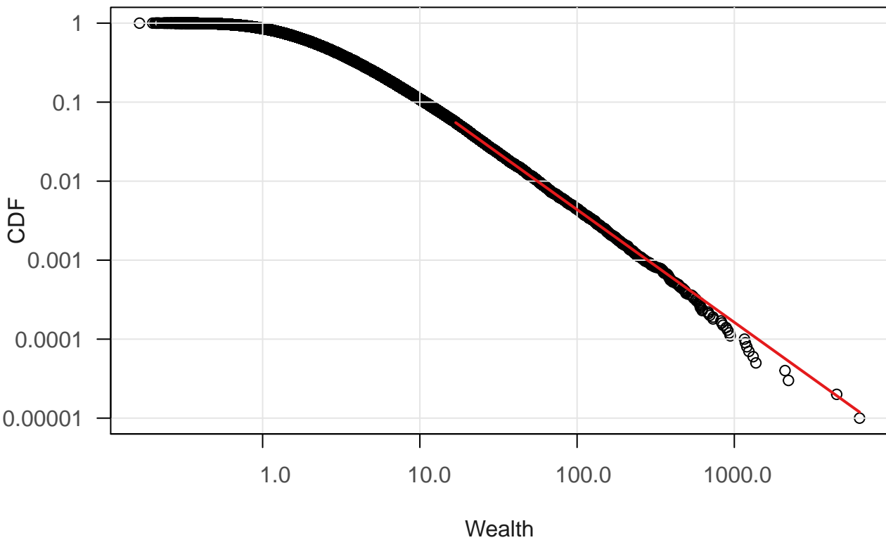
CCDF of Wealth with Power-Law Fit
