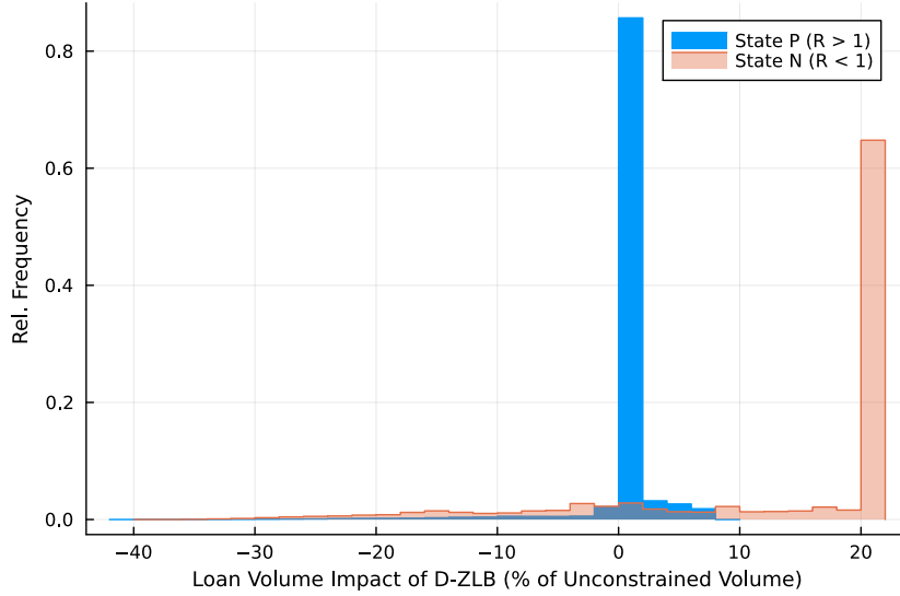
Figure 9: Histogram Loan Supply Differences (Low Deposit Model of Section A.5)
