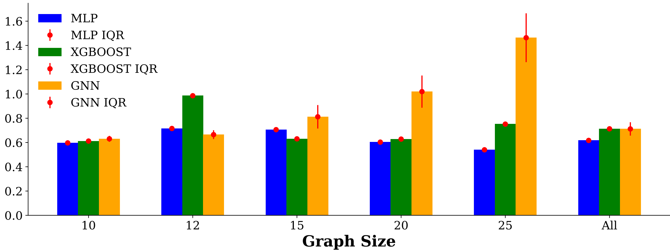
Median RMSE
