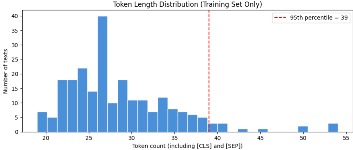
Figure 2 : Token Length
