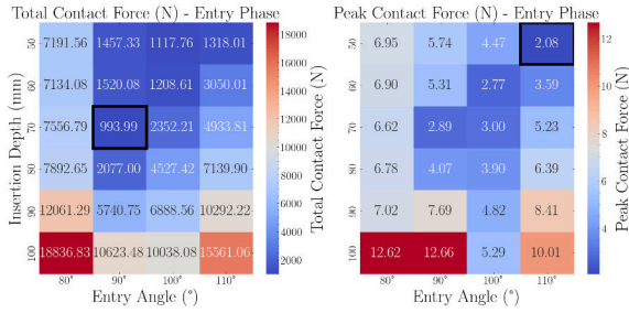
Fig. 5: Force Analysis Results – Entry Phase
