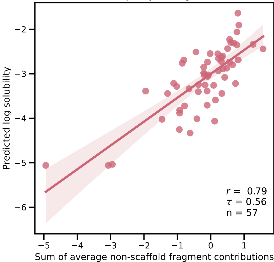
RF model: phenyl analogue series
