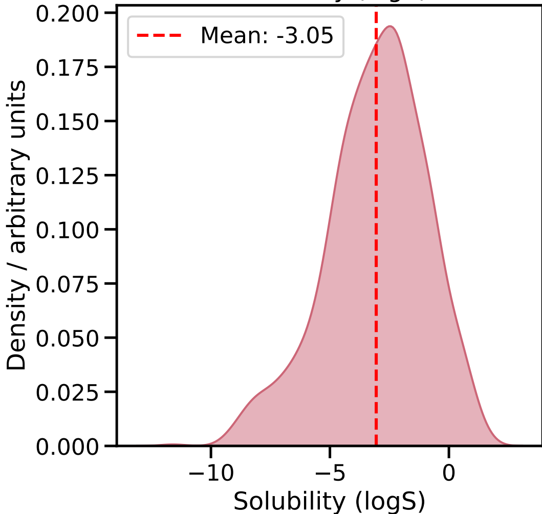
Distribution of Solubility ( \log S ) in the data
