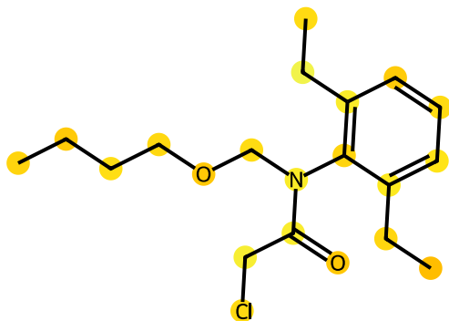
GNNExplainer
