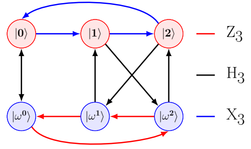
Figure 2: The Fourier-model \mathcal{F} on a qutrit. The coloring of the vertices indicate the eigenstates of X, Z .
