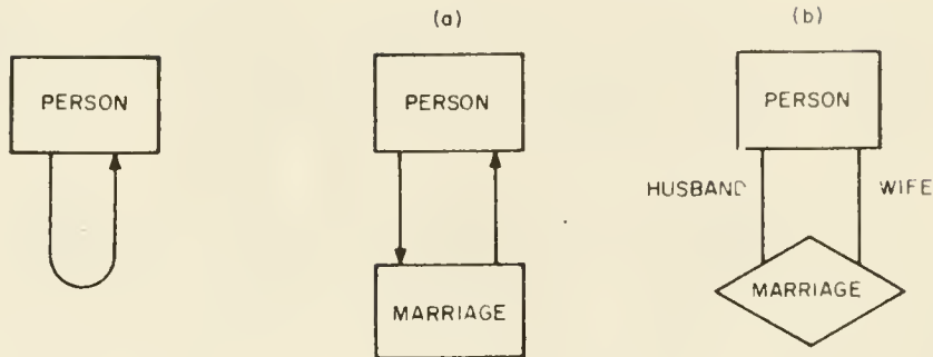
Fig. 18. Data-structure-set defined on the same record type
