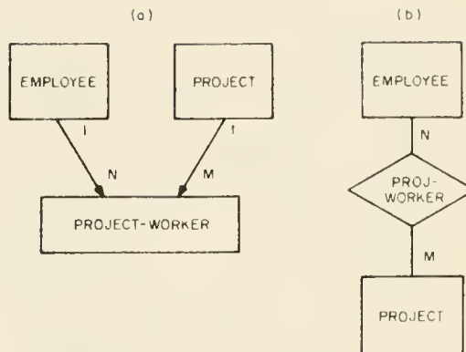
Fig. 17. Relationship PROJECT-WORKER
