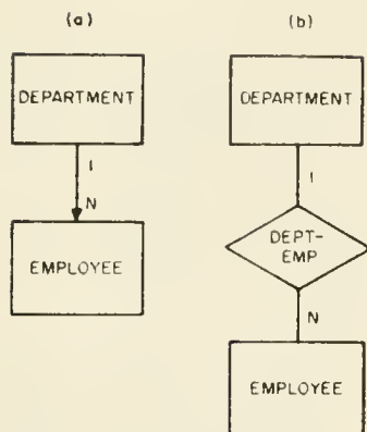
Fig. 16. Relationship DEPARTMENT-EMPLOYEE
