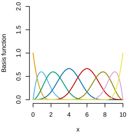
(a) B-spline basis
