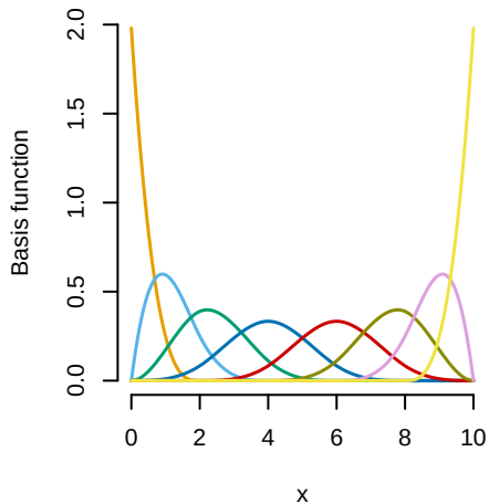
(b) Normalised basis
