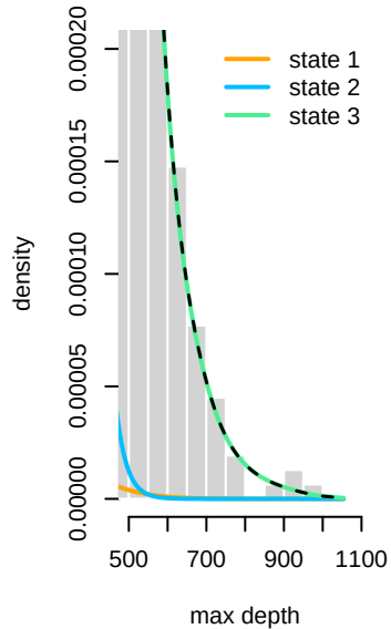
constrained
