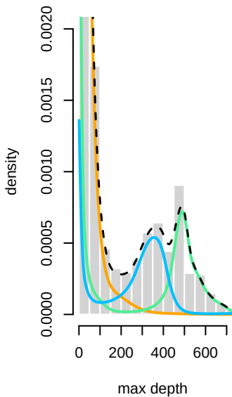
unconstrained
