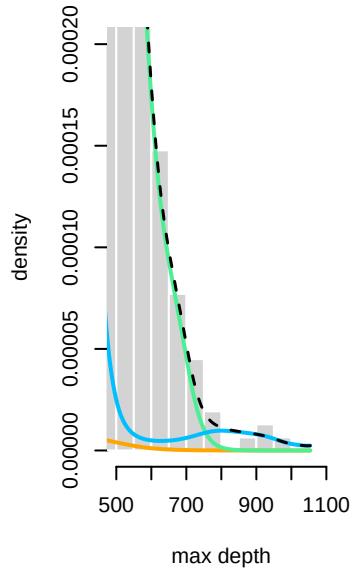
unconstrained
