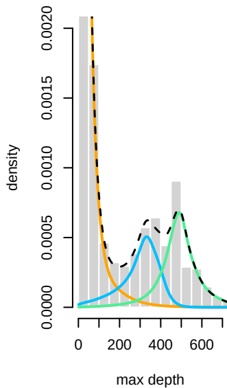
constrained
