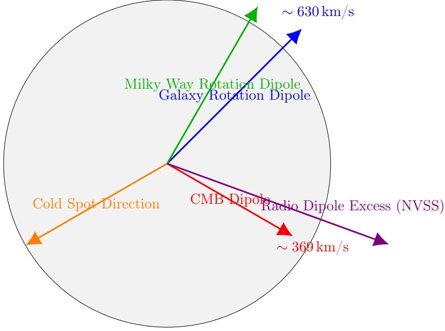
Schematic directions (based on Shamir/CMB/NVSS data)
