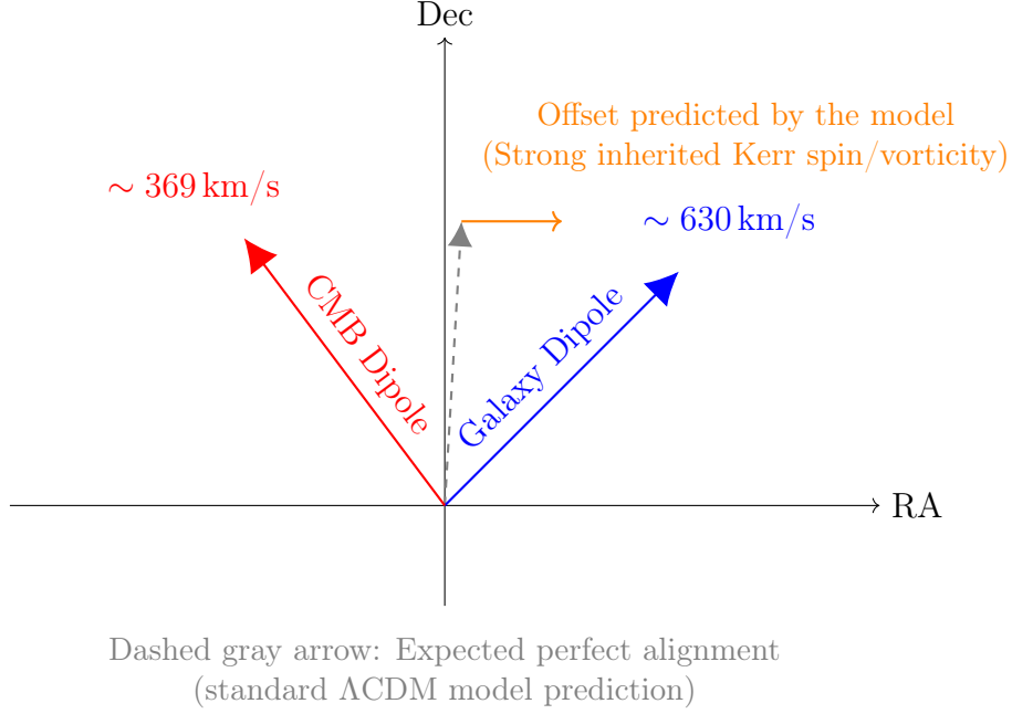
Figure 3: Galaxy rotation dipole (blue) and CMB dipole (red) in Cartesian coordinates. The dashed gray arrow shows the perfect alignment expected in the standard model, while the visible offset (orange arrow) is the present model’s prediction due to strong inherited Kerr spin and vorticity—this strengthens the model’s argument for inherent asymmetry (Shamir vs. CMB data).
