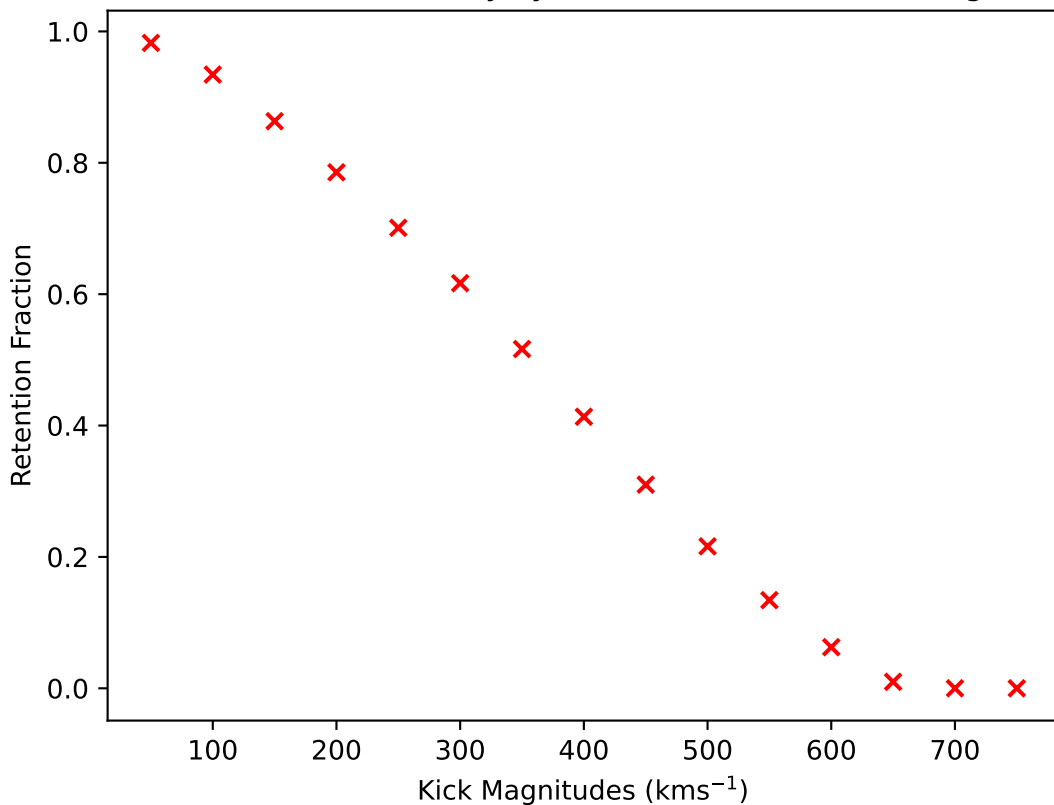
Retention fraction of binary systems (10000) vs kick magnitudes
