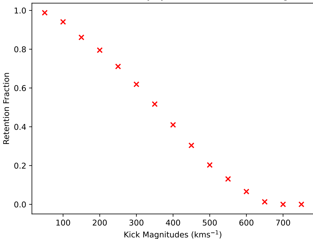
Retention fraction of binary systems (1000) vs kick magnitudes
