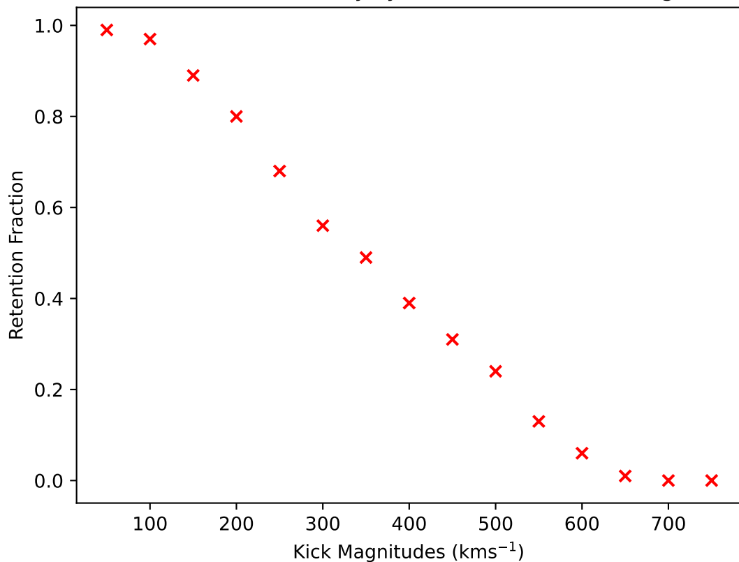
Retention fraction of binary systems (100) vs kick magnitudes
