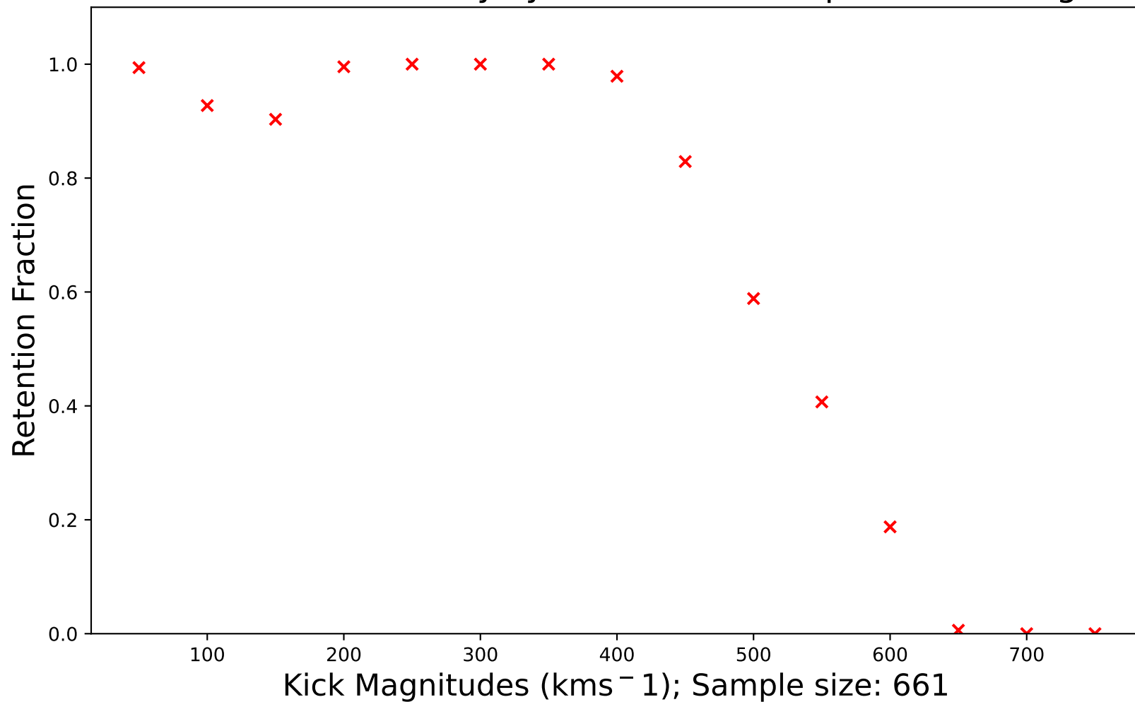
Retention fraction of binary systems within 1 kpc vs kick magnitudes
