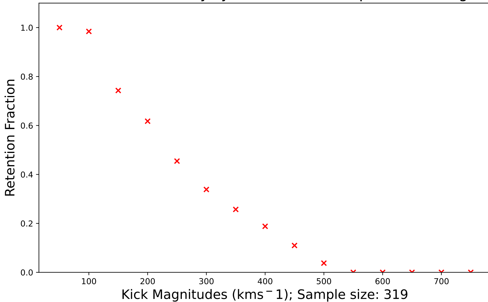
Retention fraction of binary systems within 10 kpc vs kick magnitudes
