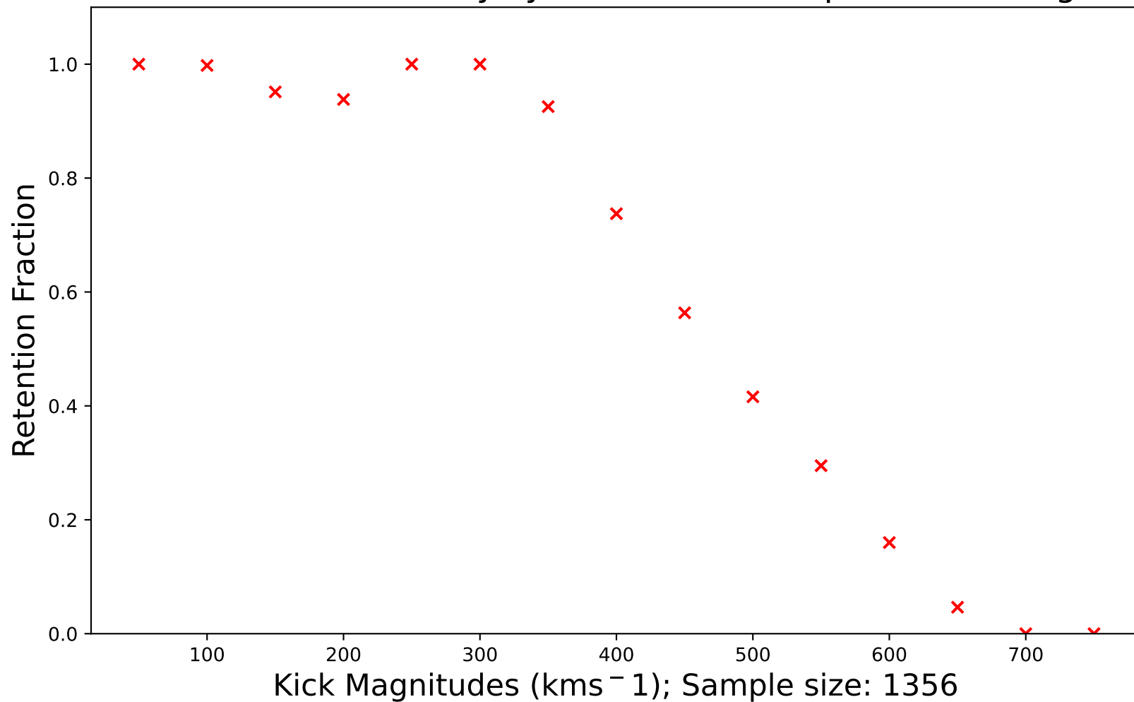
Retention fraction of binary systems within 2 kpc vs kick magnitudes
