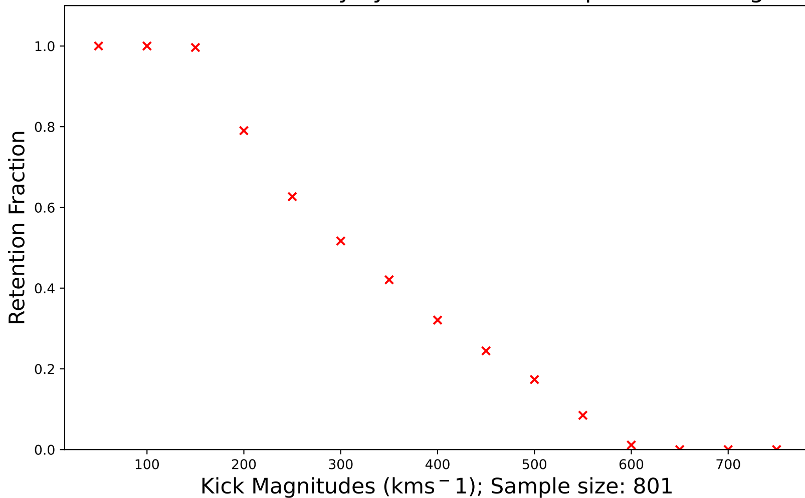
Retention fraction of binary systems within 6 kpc vs kick magnitudes
