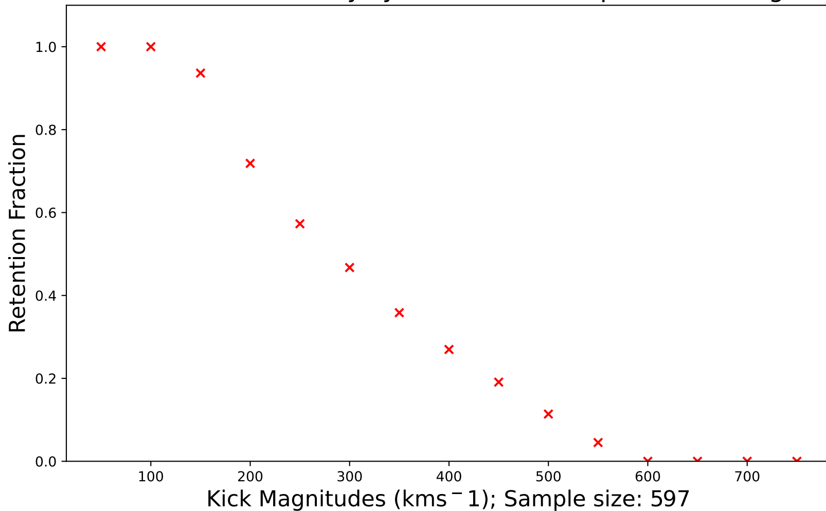
Retention fraction of binary systems within 7 kpc vs kick magnitudes
