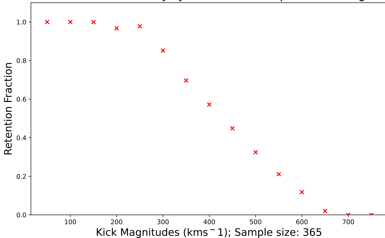
Retention fraction of binary systems within 9 kpc vs kick magnitudes
