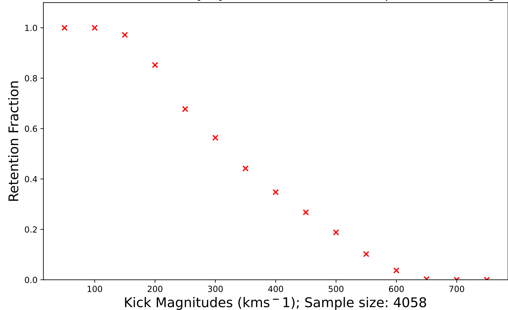
Retention fraction of binary systems between 3-8 kpc vs kick magnitudes
