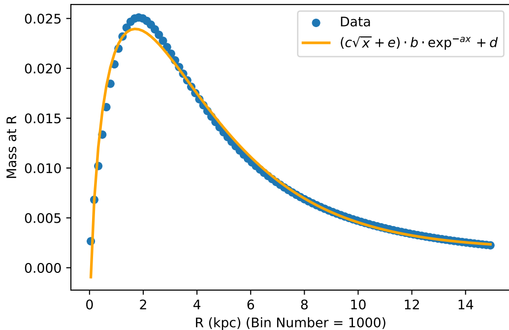
Baryonic Mass enclosed for MWPotential2014 with fit
