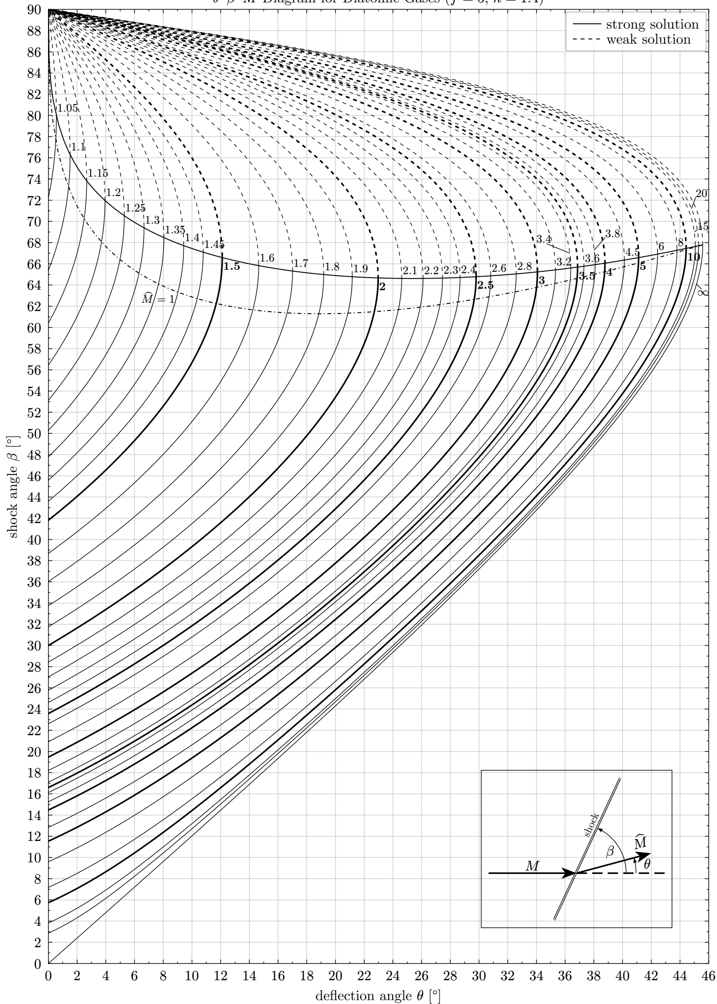
\theta - \beta - M Diagram for Diatomic Gases ( f = 5 , \kappa = 1.4 )
