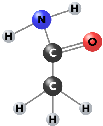
Molecular structure
