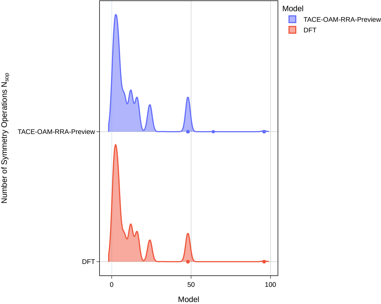
Number of Symmetry Operations in ML-relaxed Structures
