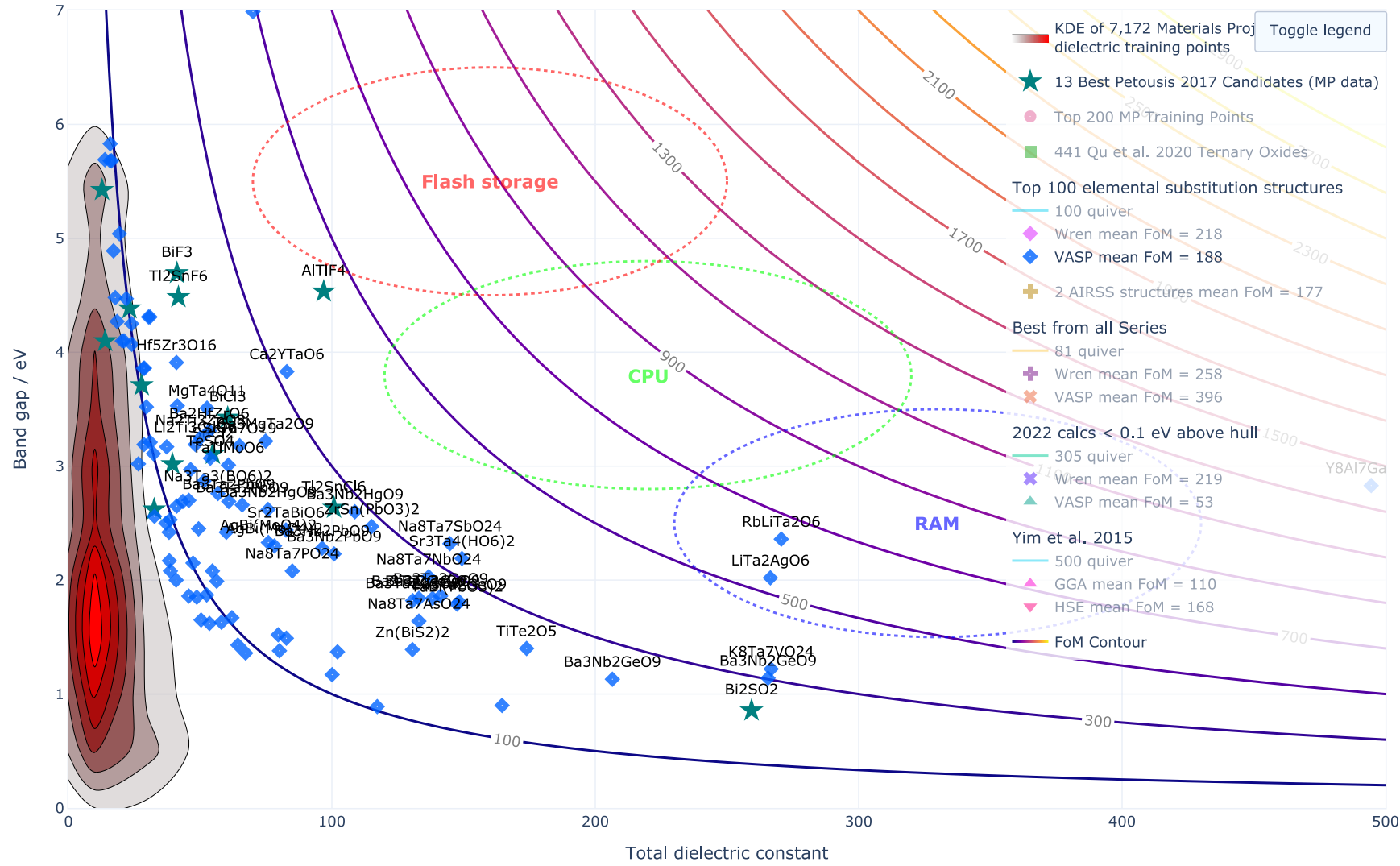
Pareto Frontier of Dielectric Constant and Band Gap - data as of 2023-10-14 20:35
