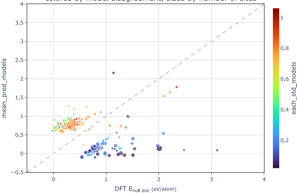
200 chalcogenides with largest hull distance errors colored by model disagreement, sized by number of sites
