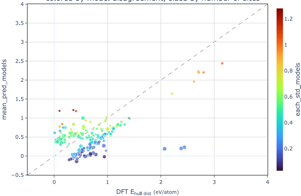
200 nitrides with largest hull distance errors colored by model disagreement, sized by number of sites
