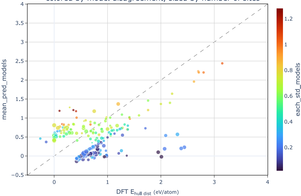
200 oxynitrides with largest hull distance errors colored by model disagreement, sized by number of sites
