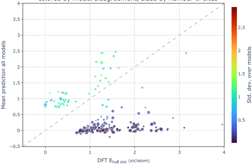
200 structures with largest hull distance errors colored by model disagreement, sized by number of sites
