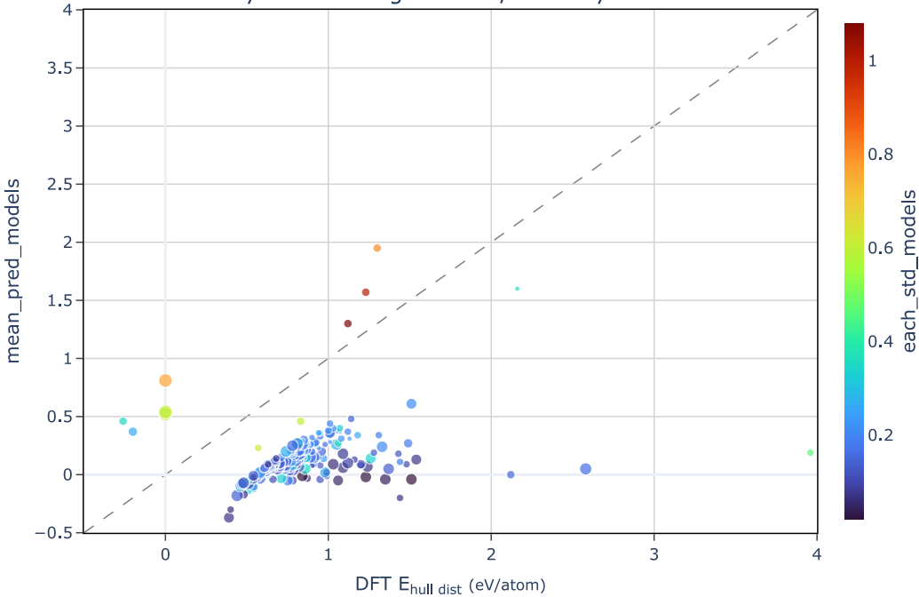
200 actinides with largest hull distance errors colored by model disagreement, sized by number of sites
