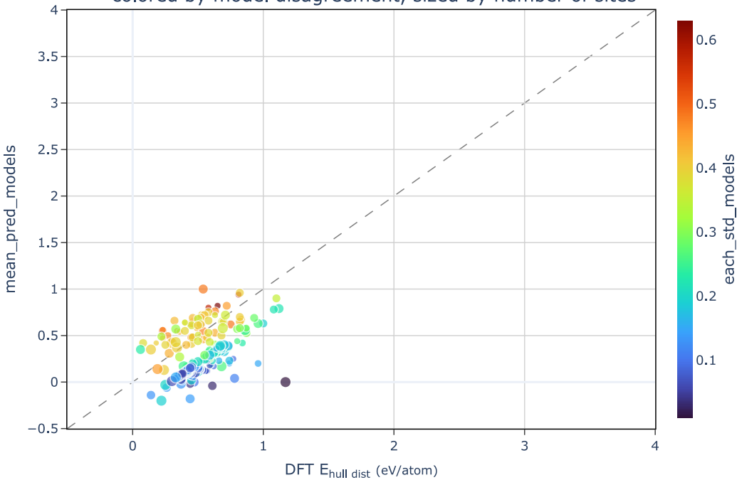
200 borides with largest hull distance errors colored by model disagreement, sized by number of sites
