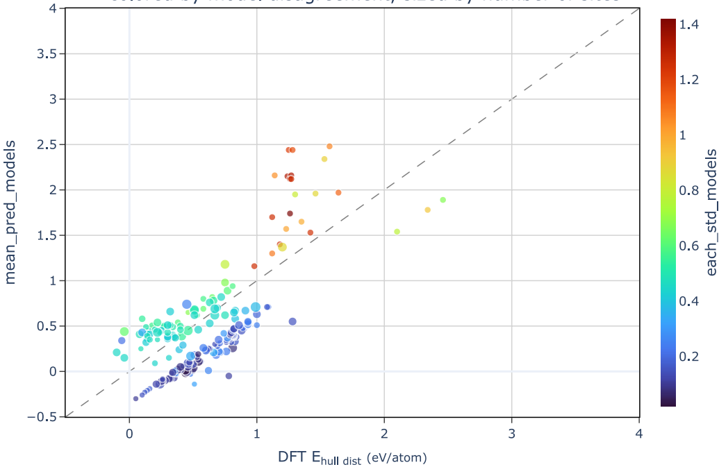
200 carbides with largest hull distance errors colored by model disagreement, sized by number of sites
